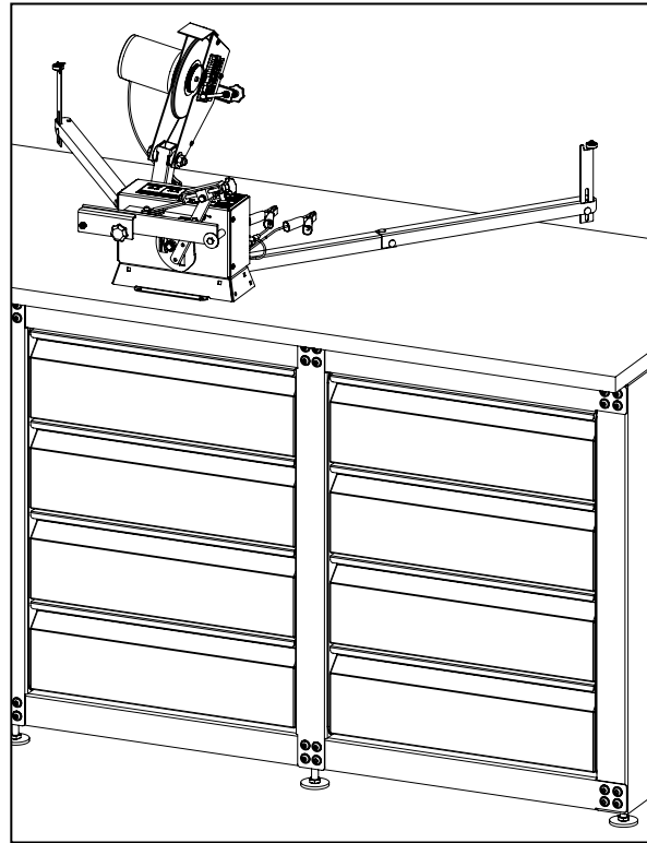
WORKBENCH MOUNT
