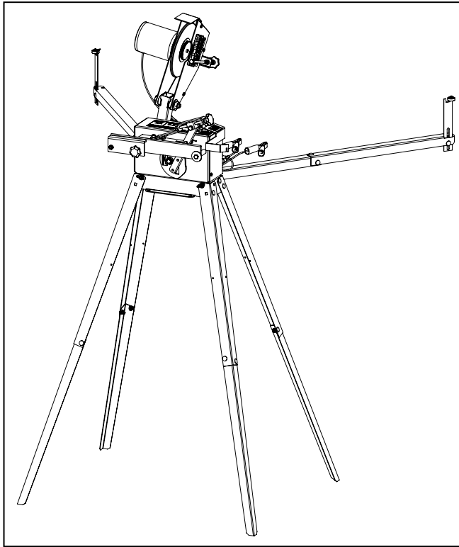
STAND MOUNT
