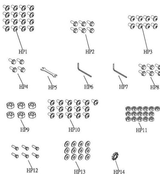
Figure 2: hardware package (not to scale)
